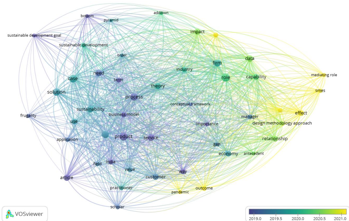
Figure 5. Overlay Visualization
