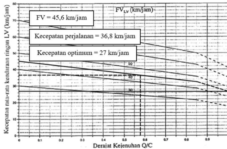
Figure 9. Optimum speed and travelling speed without markets
