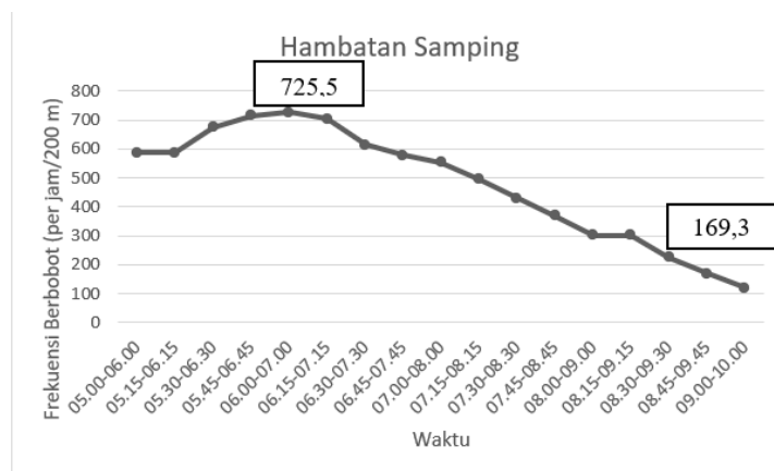
Figure 8. Side barriers
