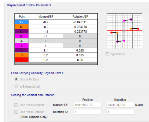
Figure 6. Plastic Joint of Beam 25/40 [12]
