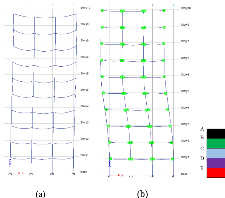
Figure 10. (a) distribution of plastic joints for the I_e/R scale and (b) Plastic joints for earthquake scale of 1
