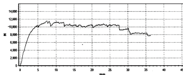
Figure 6. Cylinder compression graph with TDS328 fiber (28 days) with P_{\max} 11,517 N at d 6.75 mm and d_{\max} 36.5 mm at P 7,900 N
