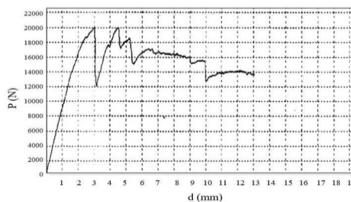
Figure 5. Deformation graph of TTS328 fiberless cylinder (28 days) with d 4.30 mm at P_{\max} 19,922 N and d_{\max} 13 mm at P 13,750 N
